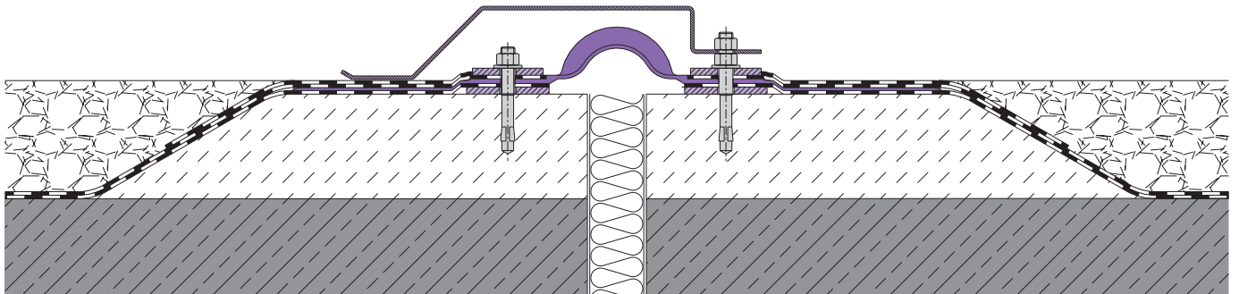
WFB 550/F
